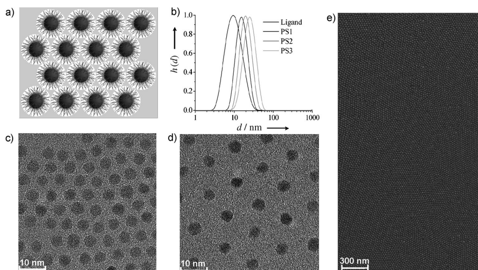
Figure 1. a) Schematic diagram of a nanocomposite consisting of nanoparticles coated with brush-like layers. b) Hydrodynamic diameters of CdSe nanoparticles coated with polystyrene of different molecular weights. PS1 3 200 g mol -1 , PS2 7 600 g mol -1 , PS3 15 600 g mol -1 . c, d) TEM images of Fe 3 O 4 nanoparticles covered with a layer of oleic acid directly after synthesis (c) and coated with a layer of polystyrene (PS2 7 600 g mol -1 ) after ligand exchange (d). The increased distance between the nanoparticles can be clearly observed. e) SEM image of a large sample area showing the stability of the nanoparticles against aggregation at high nanoparticle volume fractions.
